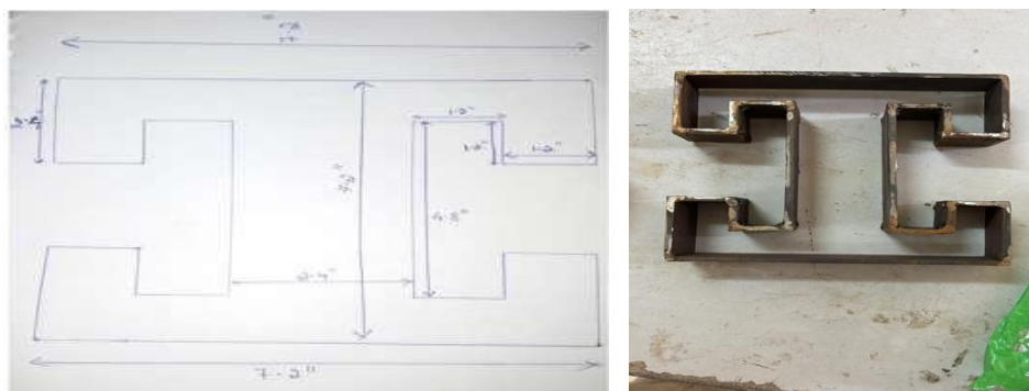
Fig 5: Dimensions and shape of the paver block
