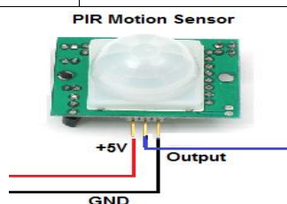
Fig 3: PIR Sensor
