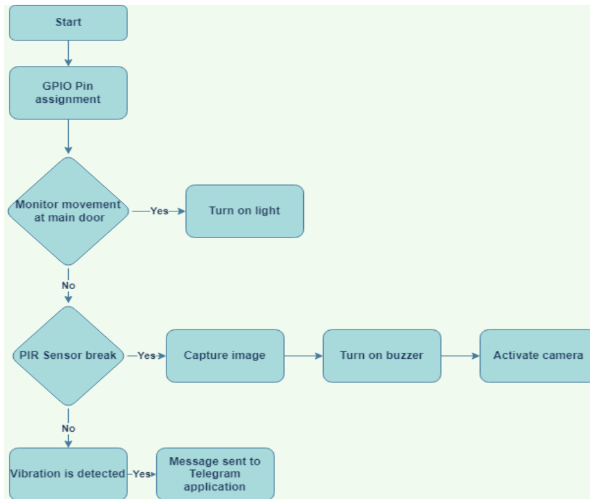
Fig 8: Flowchart of home security
