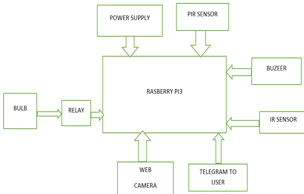
Fig 1: Block diagram of Home Security and Automation using IOT
