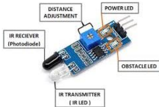
Fig 7: IR Sensor
